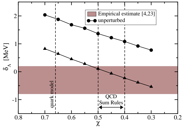
Fig. 2. Evolution of the spin-orbit splitting \delta_\Lambda = \epsilon_\Lambda(1p_{1/2}^{-1}) - \epsilon_\Lambda(1p_{3/2}^{-1}) for {}^{16}_\Lambda O as function of the ratio \chi between background scalar-vector self-energies of \Lambda vs. nucleon. The dashed line at \chi = 2/3 marks the simple quark model value. Also indicated is the \chi interval suggested by a QCD sum rule analysis [20,21]. Calculations with (without) the chiral SU(3) spin-orbit correction (11) are denoted by triangles (circles). The shaded area represents an estimate of \delta_\Lambda ( -0.8 \text{ MeV} \leq \delta_\Lambda \leq 0.2 \text{ MeV} ) based on the measured excitation energy difference \Delta E(0^+ - 2^+) in {}^{16}_\Lambda O [4,23]. This estimate is consistent with recent results from hypernuclear \gamma ray spectroscopy [5].
