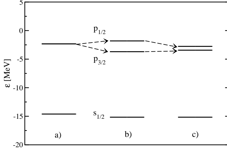
Fig. 1. \Lambda single particle energy levels in ^{16}_{\Lambda}O . Case a : using the single particle potential based on the density dependent coupling strengths including chiral K and 2\pi exchange as determined in Ref. [13] (see Sect. II). Case b : adding the spin-orbit effect from in-medium quark condensates, with reduction factor \chi = 2/3 according to a simple quark model [7]. Case c : additional compensating effect of the chiral SU(3) spin-orbit potential from the second order \Lambda N tensor force with intermediate \Sigma (see Eq.(11)).
